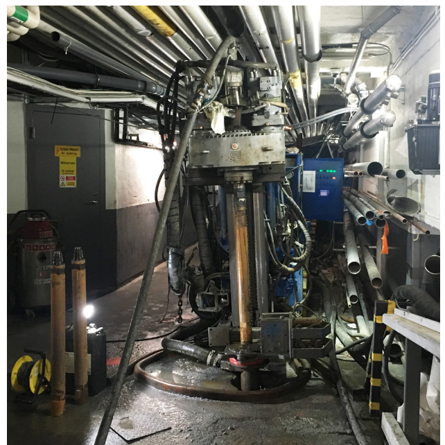
Wessman Drilling Solutions drilling in the basement of the building at Stureplan
